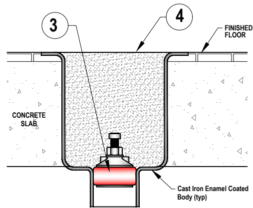
FLOOR SINK ABANDONMENT
