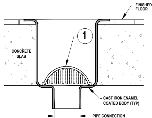
FLOOR SINK SECTION
